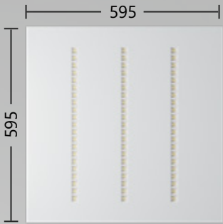
Optics:Reflector cover
